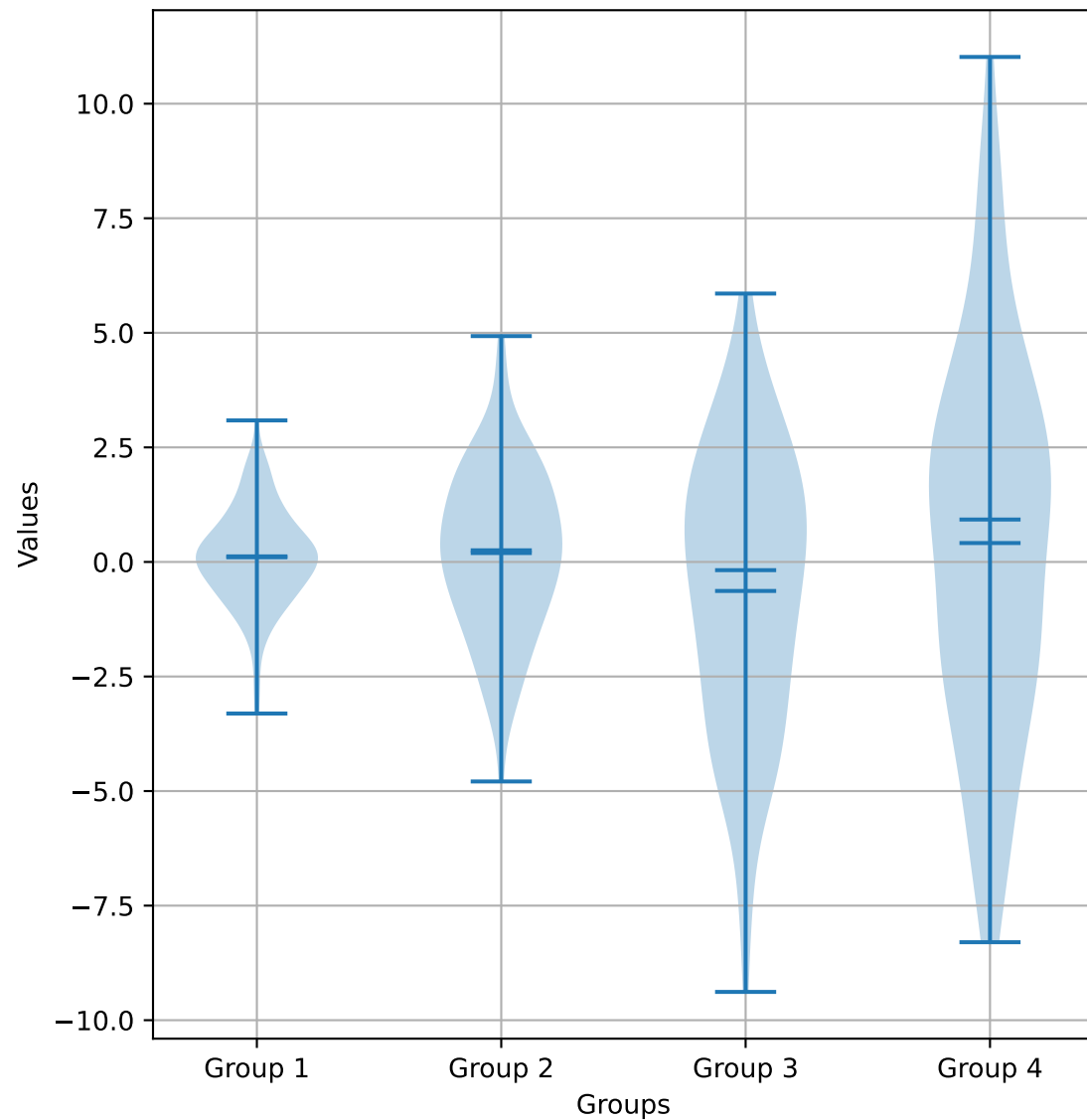
Violin Plot
