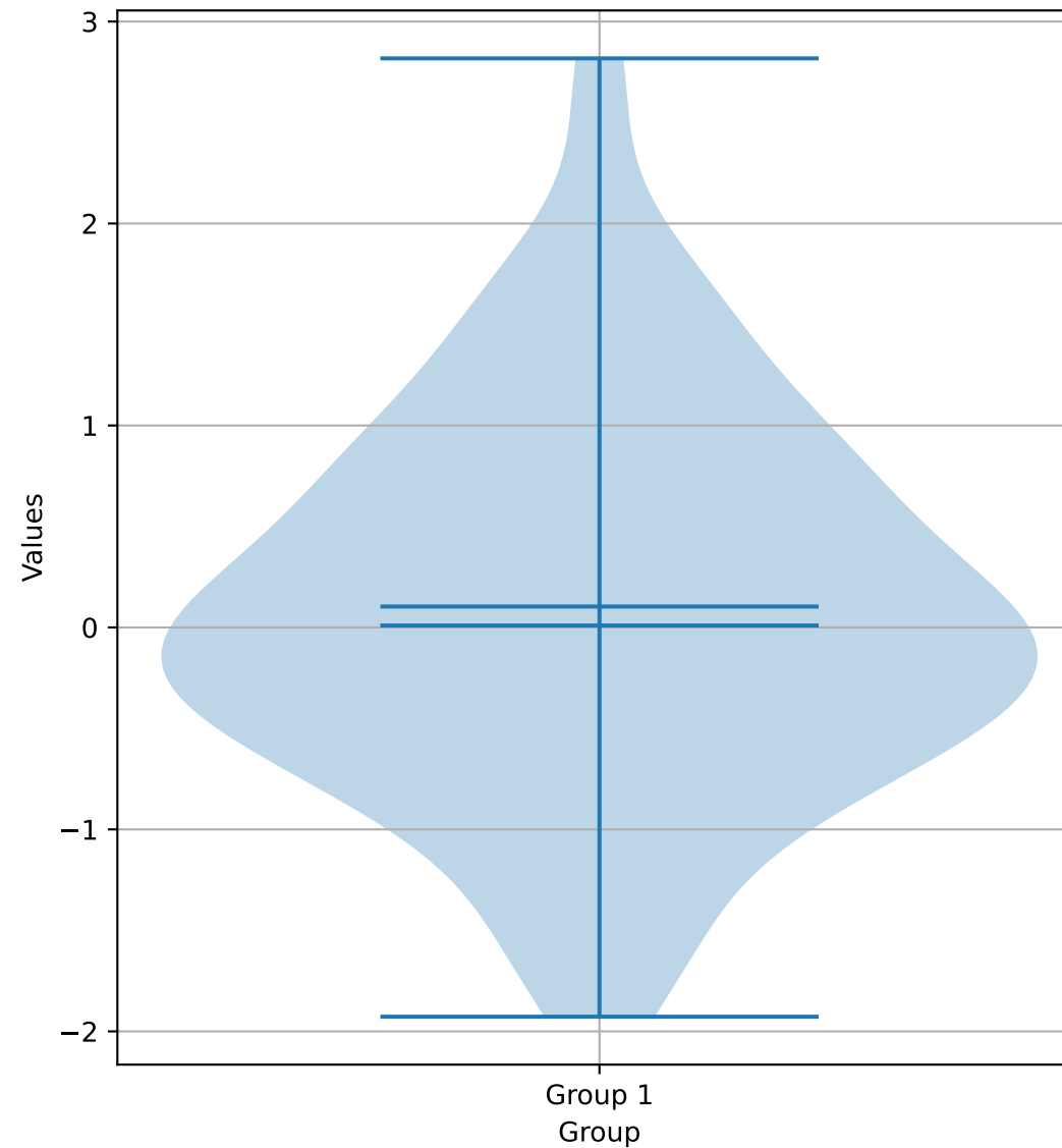
Violin Plot
