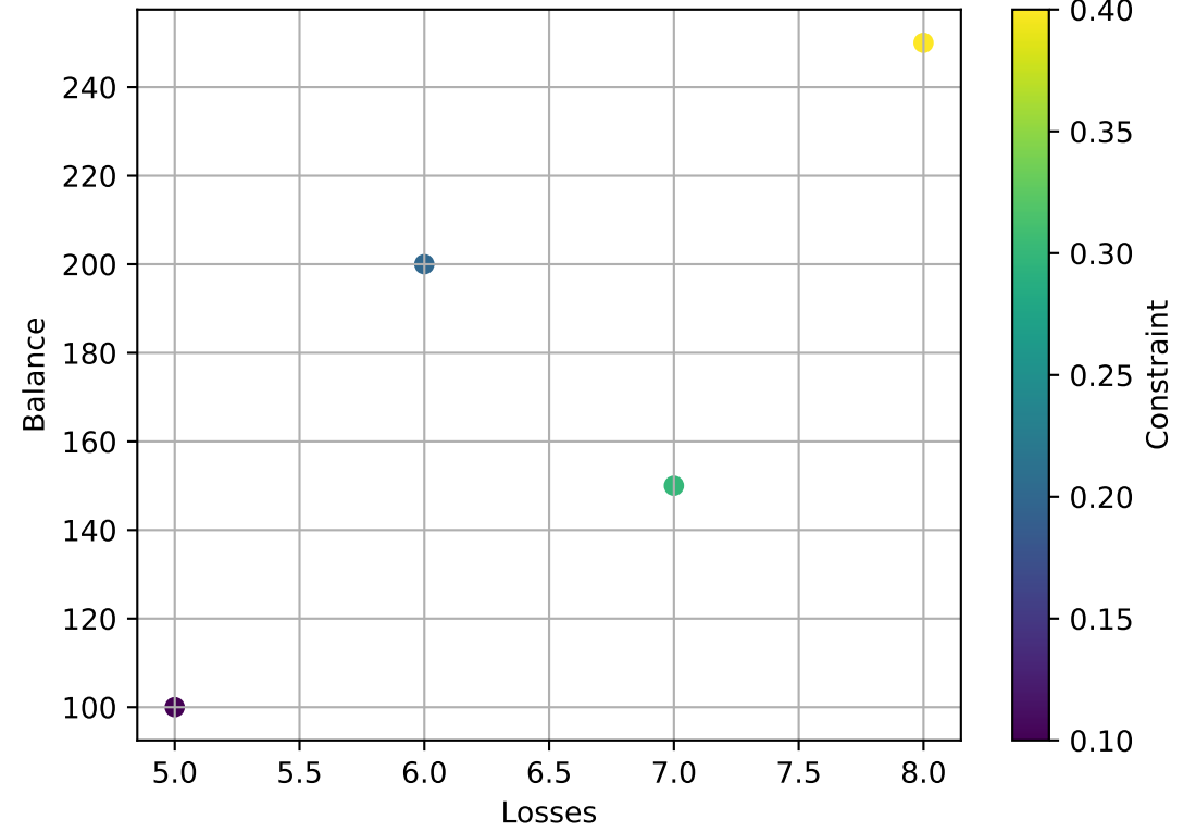
Scatter Plot
