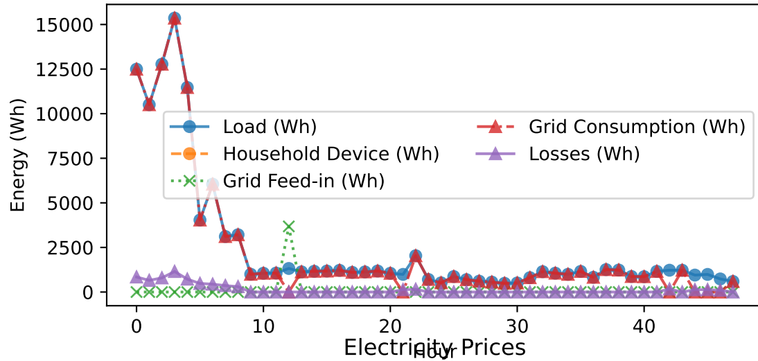
Energy Flow per Hour
