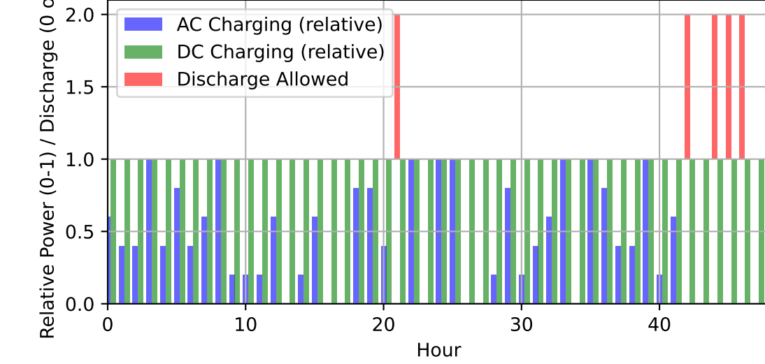
AC/DC Charging and Discharge Overview
